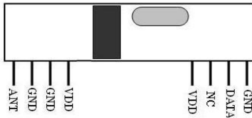
Figure1 CY33 Shape & Pins
