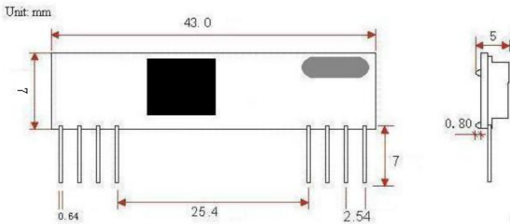
Figure2 CY33 Dimension
