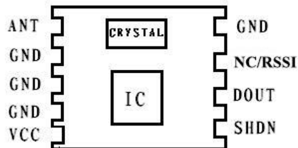
Figure1 CY88-V1.1 Shape & Pins
