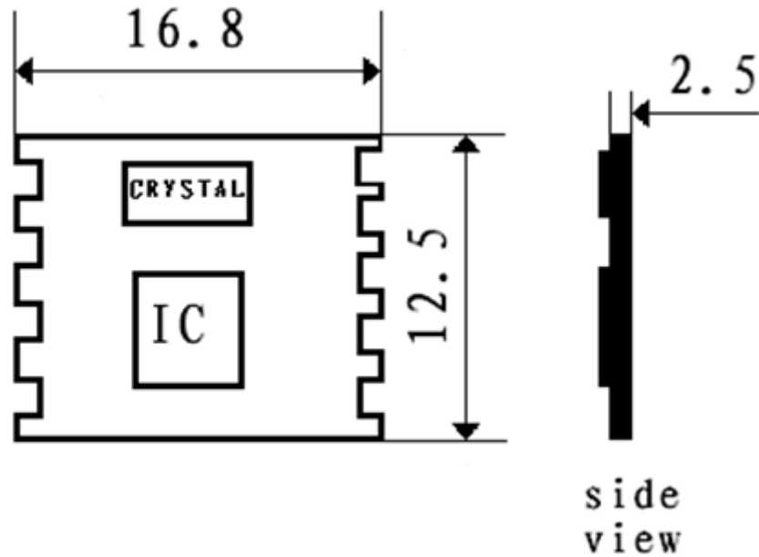
Figure2 CY88-V1.1 Dimension
